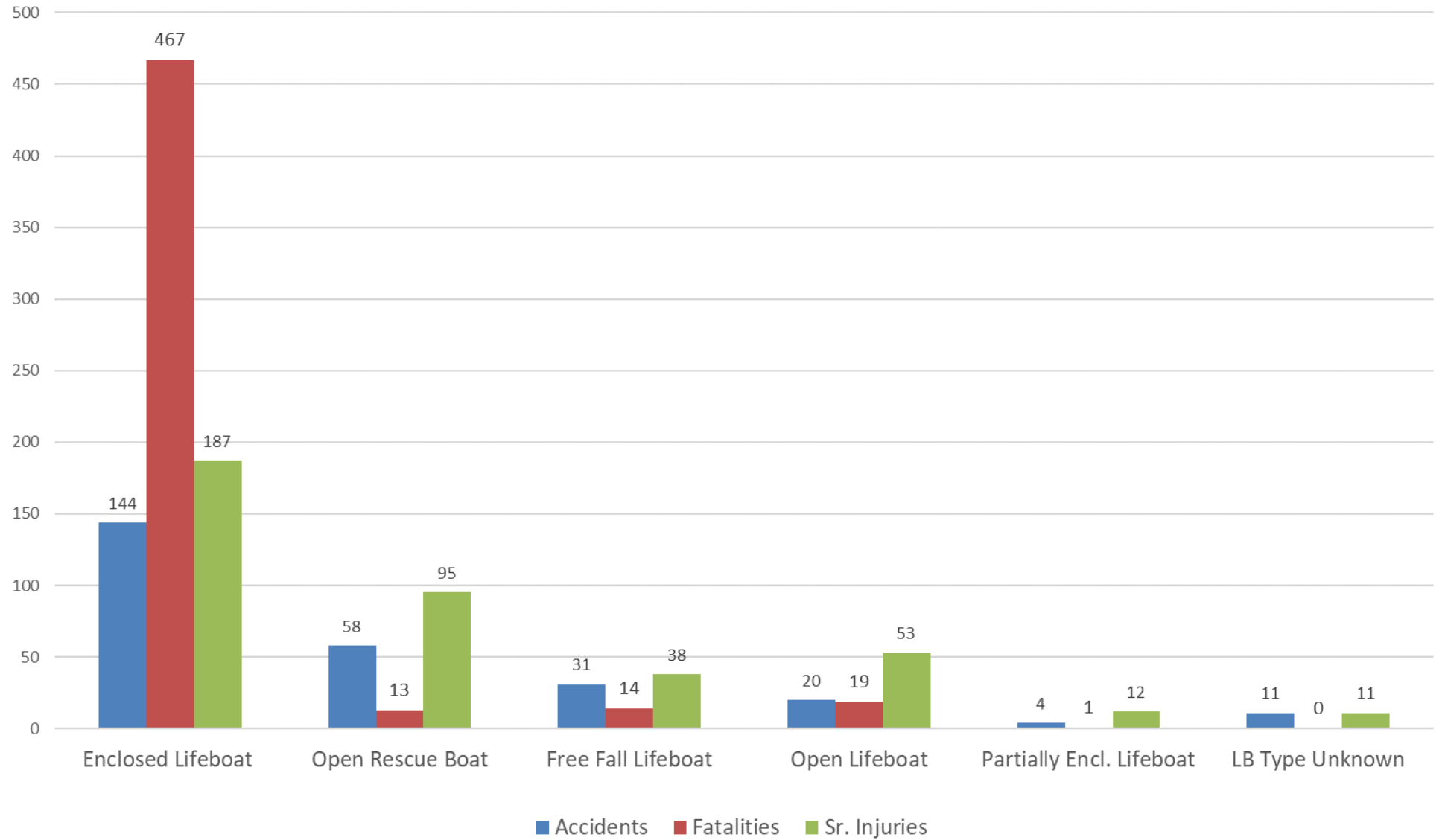
Accidents & Casualties with type of Lifeboats 1980-2023
