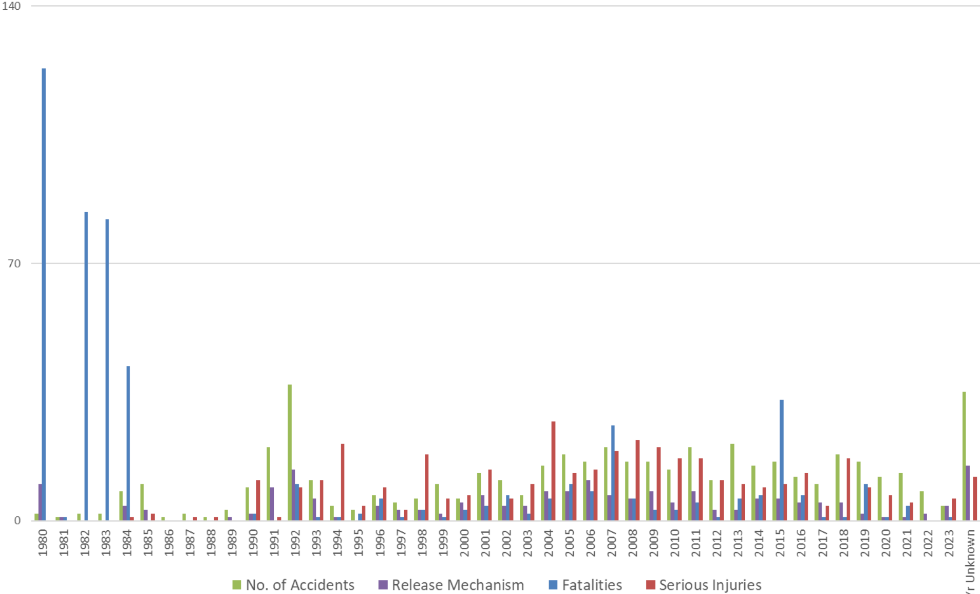
Accidents related to Release Mechanism 1980-2023
